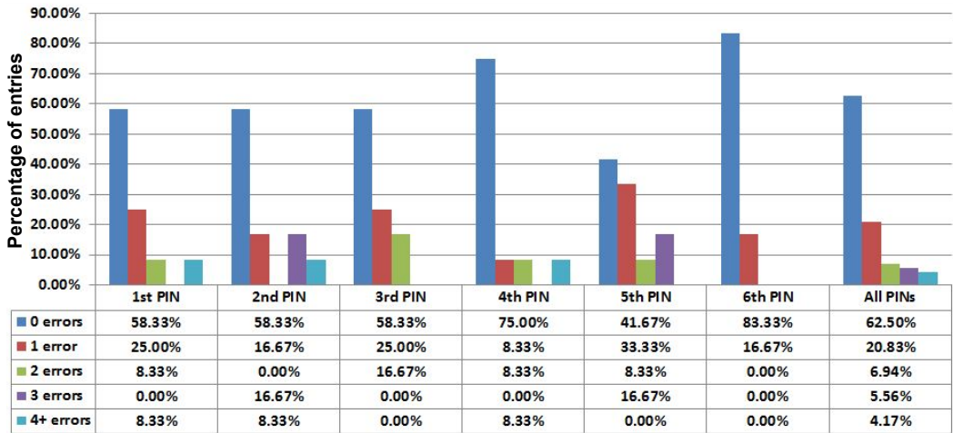
Fig. 7. Number of attempts before a successful entry using GazeTouchPIN across all participants. Each participant entered 6 PINs using GazeTouchPIN, the graph shows that users tend to enter their PIN correctly at the first attempt as they enter more PINs.
