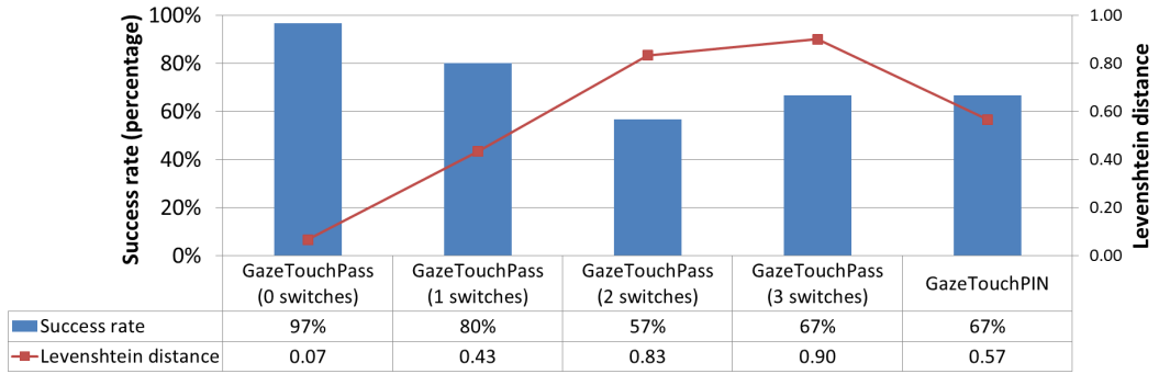
Fig. 10. The figure shows that, similar to previous work, the Levenshtein distance is larger in case of 2- and 3-switches. This means that GazeTouchPass is more secure when more switches exist in the password. GazeTouchPIN is far less secure against our threat model compared to previously studied ones, since the random layout is no longer effective when two attackers observe simultaneously. Overall, while success rates are much higher in the multiple observers threat model compared to models studied in the past, both schemes still outperform the baseline.
