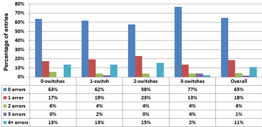
Fig. 5. Number of attempts before a successful entry. Errors are less for passwords with 3-switches; consecutive gaze gestures can be error prone, while 3-switches in an n=4 password can be only achieved by alternating gaze and touch input.
