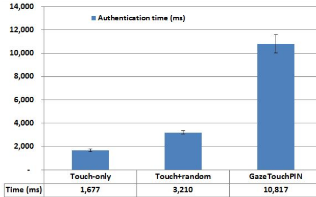
Fig. 6. GazeTouchPIN requires on average significantly more time compared to touch+random and touch-only. Participants performed faster over time, with a mean input time decreasing from 10.8 at the first GazeTouchPIN entry to 9.5 seconds at the sixth entry.
