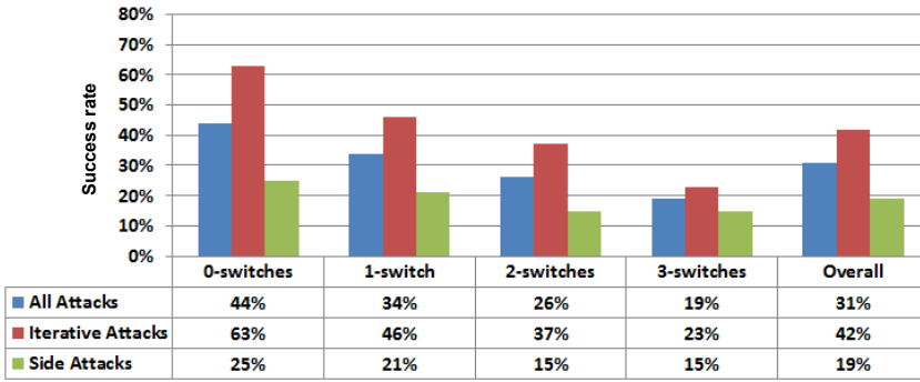
Fig. 8. Success rate when attacking passwords entered using GazeTouchPass in Security Study 1. Passwords with higher modality-switch-count are significantly more secure against observations compared to those with fewer modality-switch-count . Side attacks are always less successful than iterative attacks due to the difficulty of continuously switching focus back and forth from the eyes to the touchscreen.
