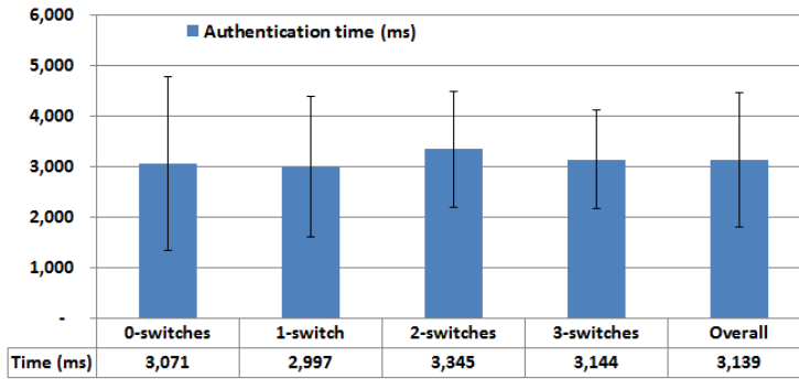
Fig. 4. Mean authentication times for passwords with different numbers of modality switches. Error bars represent the standard deviation. Authentication times do not vary significantly among different number of modality switches. Overall mean authentication time is 3.1 seconds (SD=1.3).
