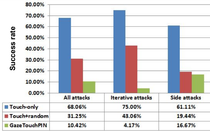
Fig. 9. Success rate of attacking PINs entered using the three methods in Security Study 2. GazeTouchPIN provided the highest level of security among the tested methods, in particular against iterative attacks.
